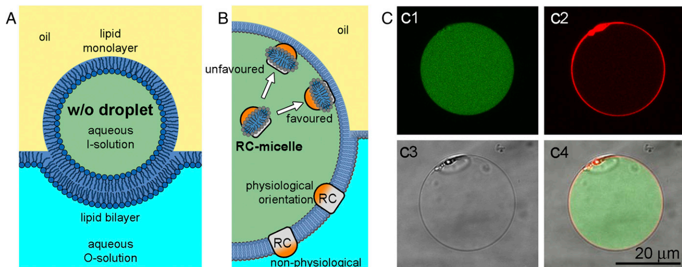
Fig. 1. Preparation of GUVs by the droplet transfer method (48). (A) Water in oil (w/o) droplets, prepared by the emulsification of an aqueous solution (I-solution) in a lipid-rich oil phase, are transferred to an aqueous solution (O-solution) by centrifugation. (B) For preparing RC@GUVs, a detergent-stabilized RC solution (RC-micelles) is emulsified in oil, giving the w/o droplets. Owing to asymmetric RC-micelle structure a preferential “physiological” RC orientation is expected, namely, with the H subunit (in orange) facing toward the aqueous core of the droplets (the cytoplasm-like GUV lumen), and the photoactive dimer (SI Appendix, Fig. S2 A and B) facing the GUV exteriors (in white). (C) RC@GUVs (POPC:POPG, 9:1) as imaged by confocal microscopy. Red-fluorescent AE-RC was reconstituted in calcein-containing GUVs. (C1) Green fluorescence channel (calcein). (C2) Red fluorescence channel (AE-RC). (C3) Bright field. (C4) Overlay of the C1, C2, and C3 channels.
